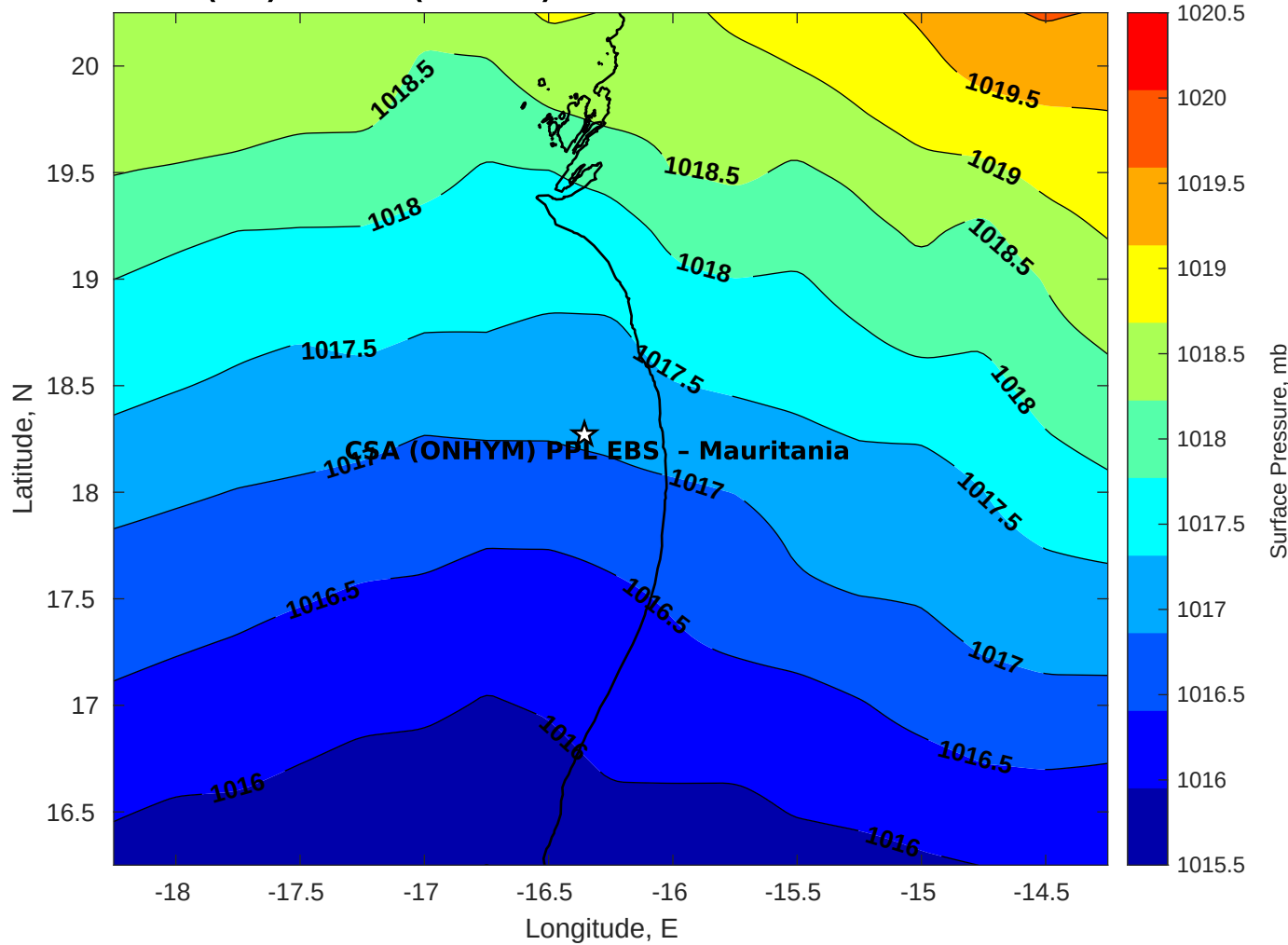
Surface Pressure (mb) for CSA (ONHYM) PPL EBS - Mauritania at 17-Feb-2026 00:00:00
