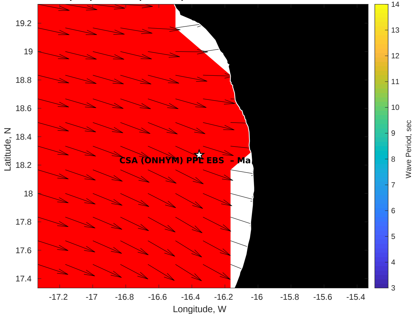
GFS Wave Period (sec) for CSA (ONHYM) PPL EBS - Mauritania at 17-Feb-2026 09:00:00
