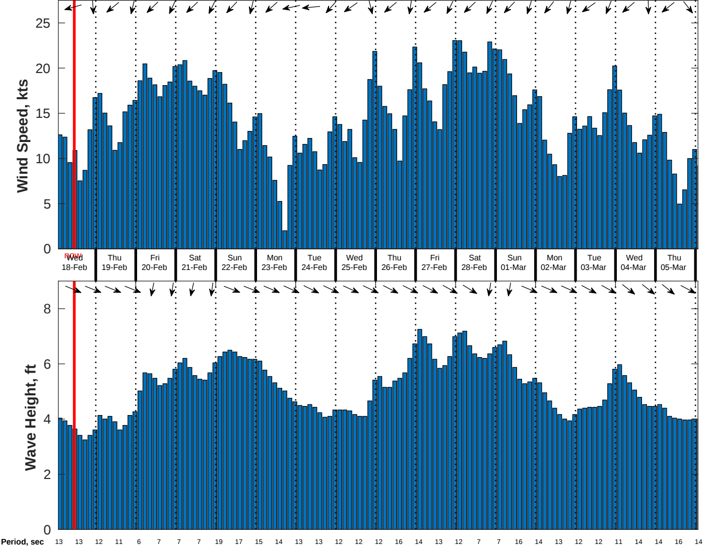
Wind & Wave Forecast for CSA (ONHYM) PPL EBS - Western Sahara from 17-Feb-2026 01:00:00 to 05-Mar-2026 01:00:00
