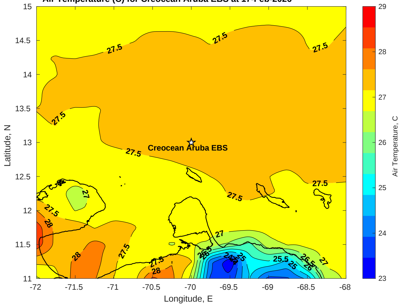
Air Temperature (C) for Creoccean Aruba EBS at 17-Feb-2026
