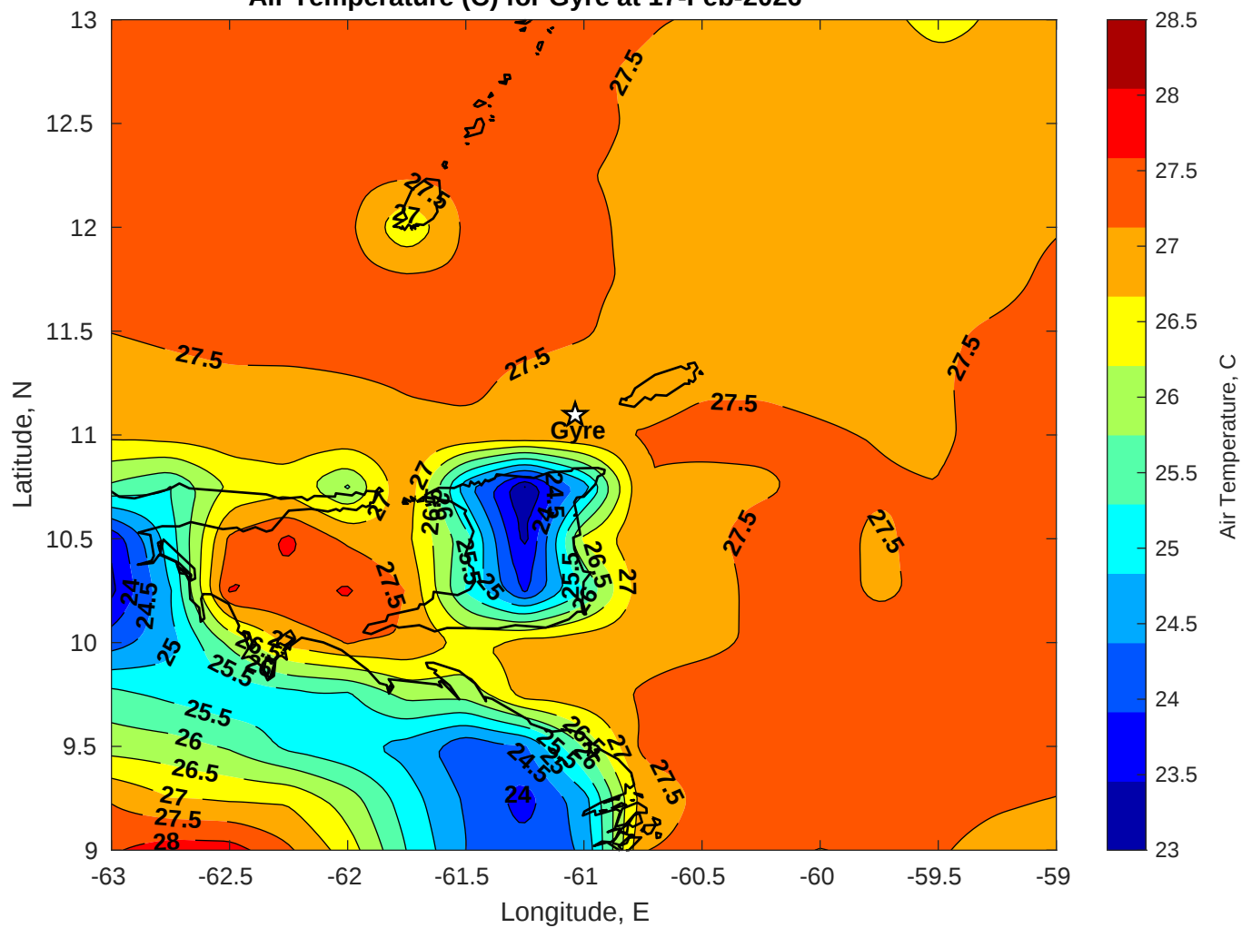
Air Temperature (C) for Gyre at 17-Feb-2026
