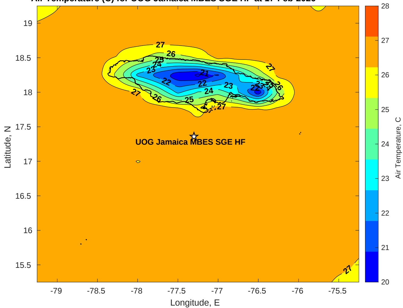
Air Temperature (C) for UOG Jamaica MBES SGE HF at 17-Feb-2026
