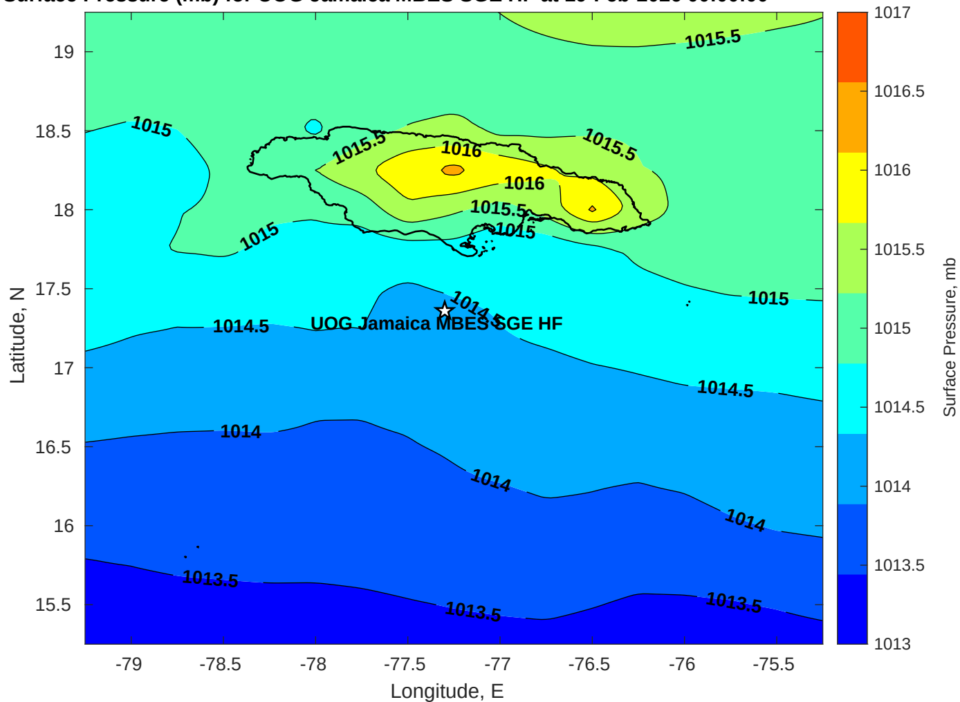
Surface Pressure (mb) for UOG Jamaica MBES SGE HF at 19-Feb-2026 00:00:00
