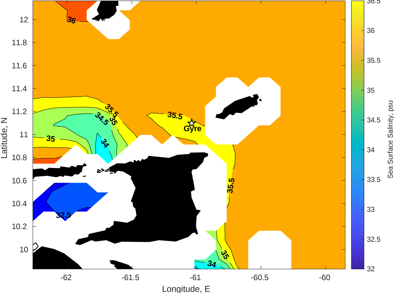
Surface Salinity for Gyre at 17-Feb-2026 00:00:00
