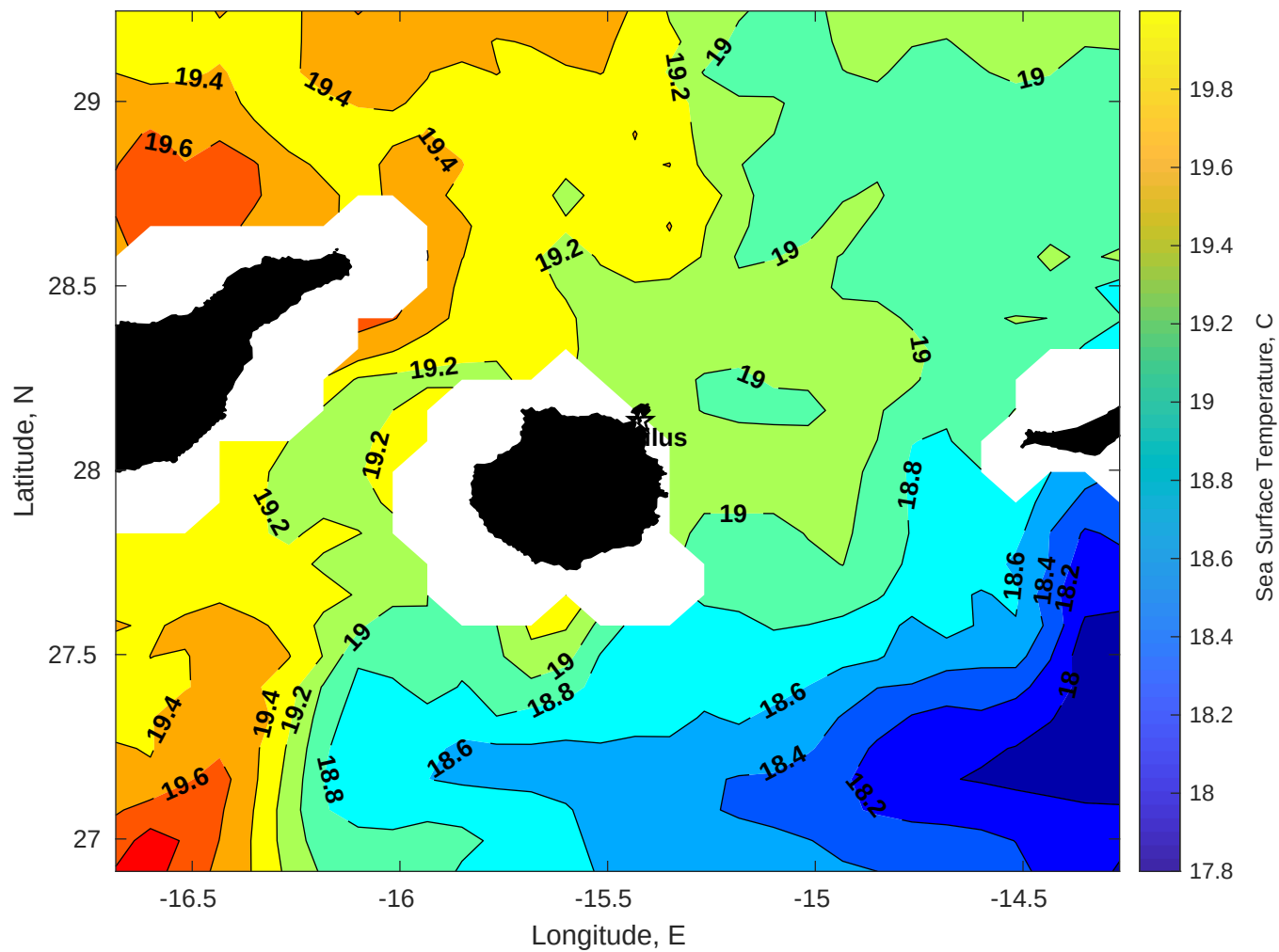
SST for Nautilus at 17-Feb-2026 00:00:00
