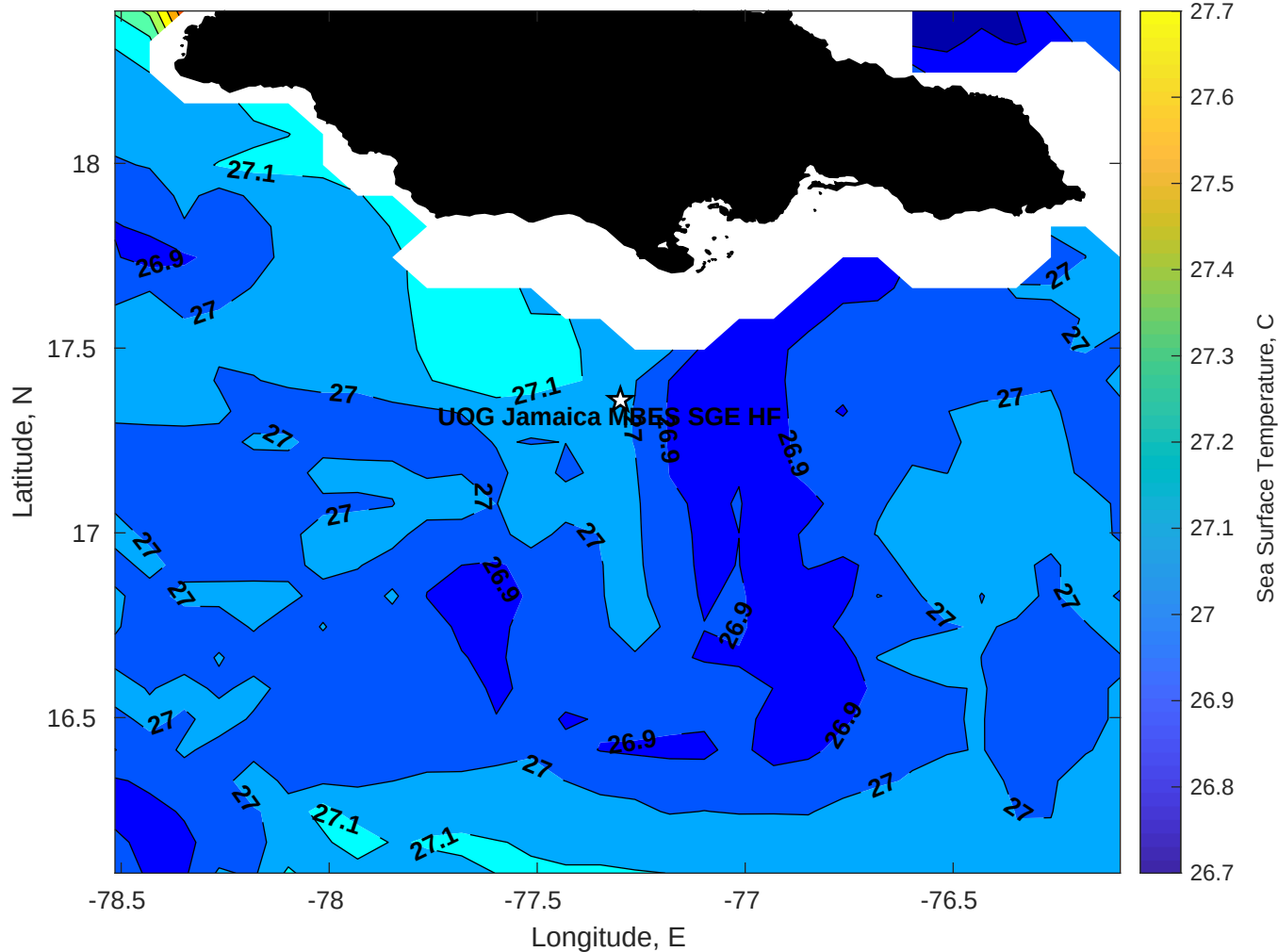
SST for UOG Jamaica MBES SGE HF at 17-Feb-2026 00:00:00
