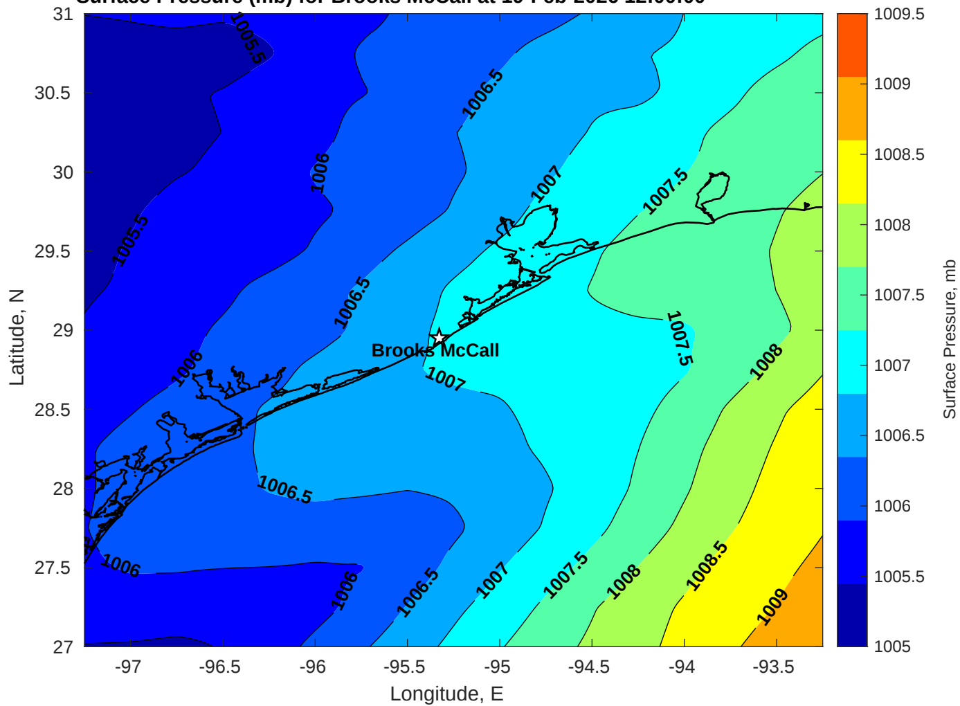
Surface Pressure (mb) for Brooks McCall at 19-Feb-2026 12:00:00
