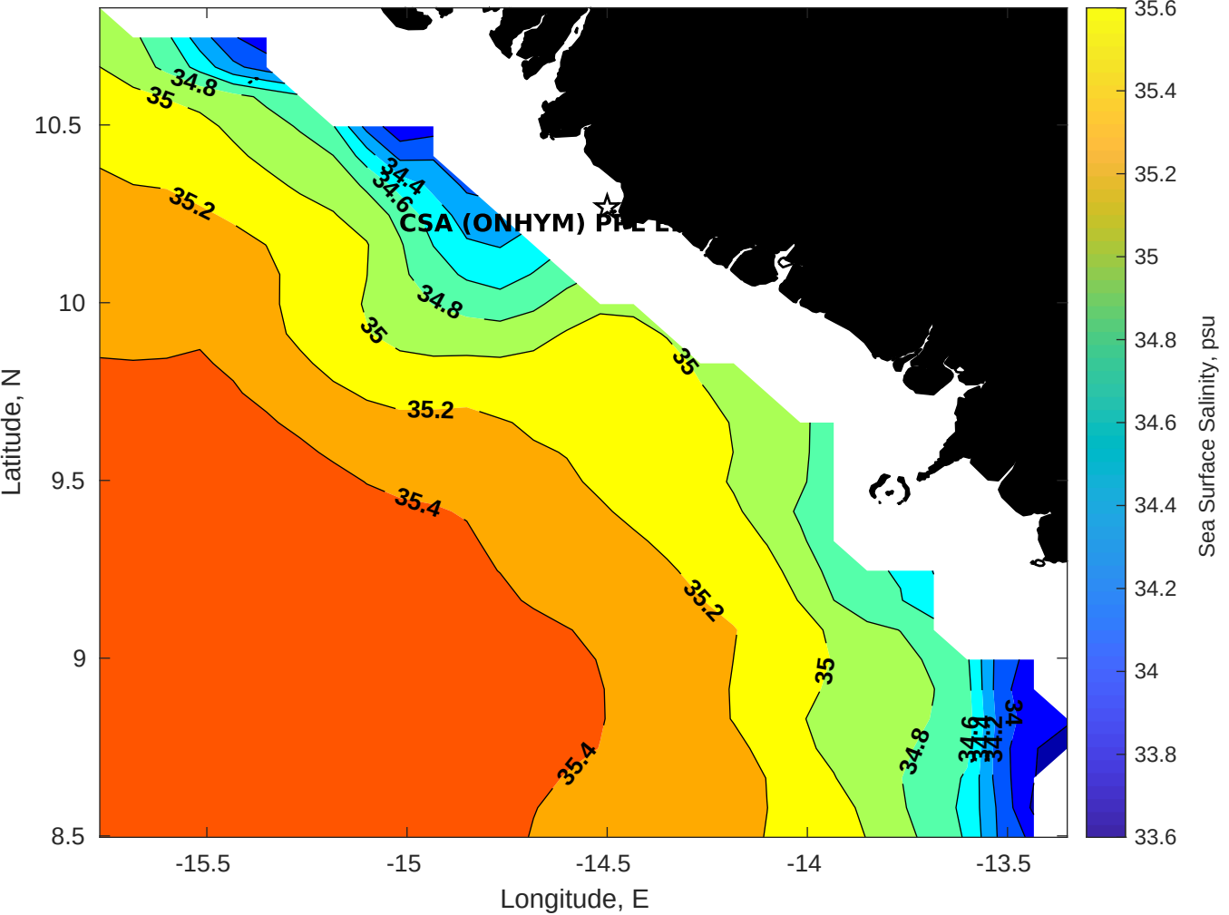
Surface Salinity for CSA (ONHYM) PPL EBS - Guinea at 18-Feb-2026 00:00:00
