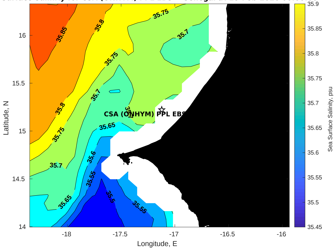
Surface Salinity for CSA (ONHYM) PPL EBS - Senegal at 18-Feb-2026 00:00:00
