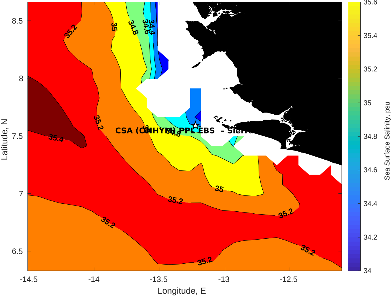
Surface Salinity for CSA (ONHYM) PPL EBS - Sierra Leone at 18-Feb-2026 00:00:00
