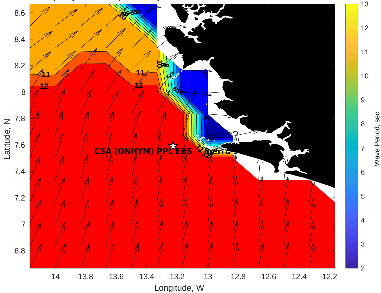
GFS Wave Period (sec) for CSA (ONHYM) PPL EBS - Sierra Leone at 18-Feb-2026 21:00:00
