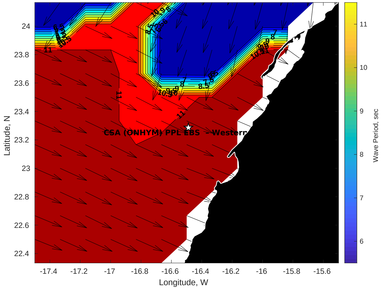
GFS Wave Period (sec) for CSA (ONHYM) PPL EBS - Western Sahara at 18-Feb-2026 21:00:00
