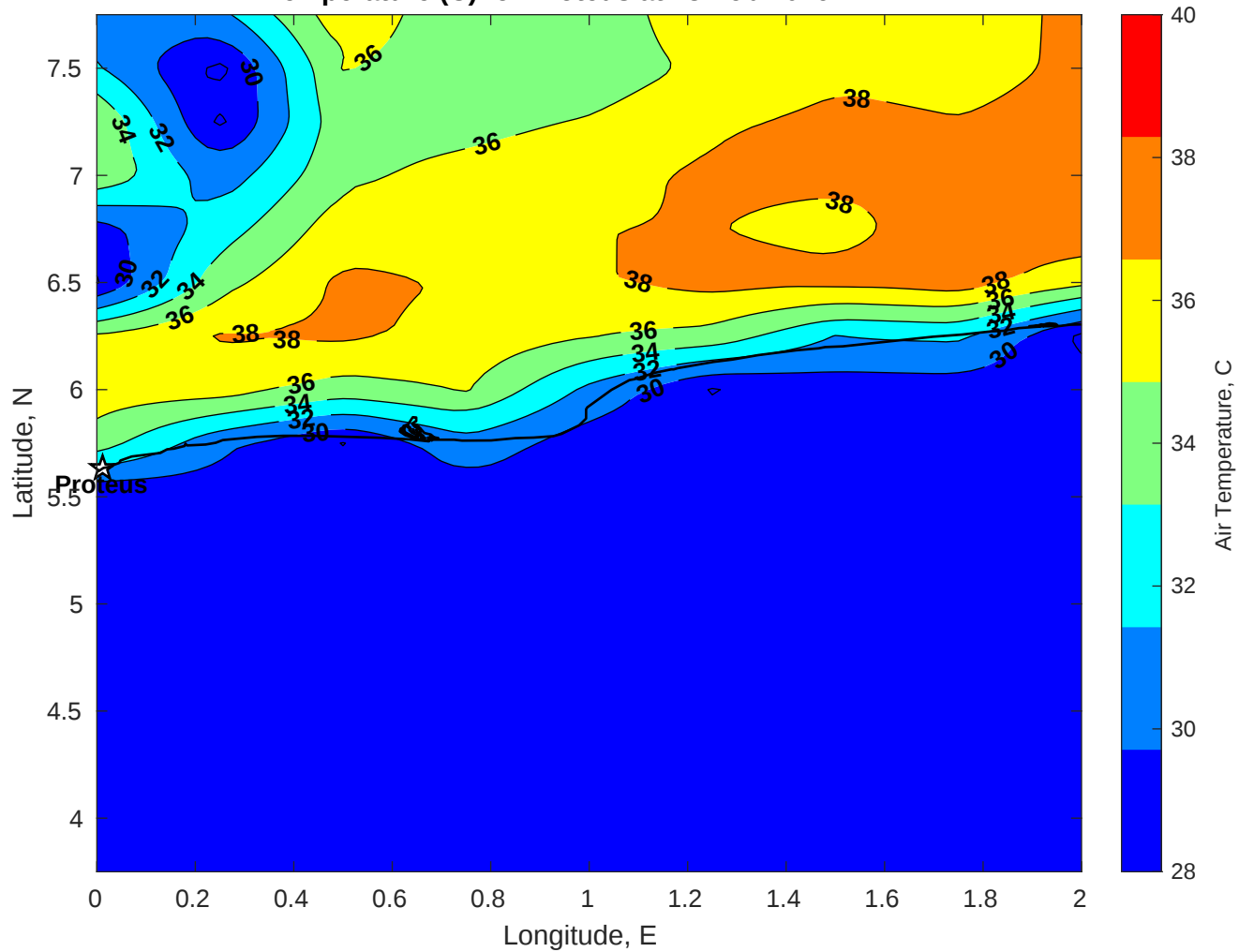
Air Temperature (C) for Proteus at 18-Feb-2026
