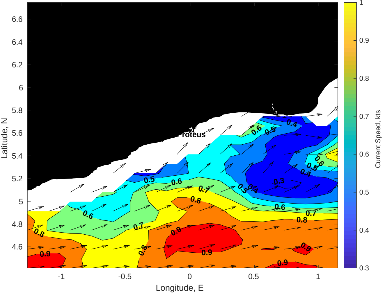
Surface Currents for Proteus at 18-Feb-2026 00:00:00
