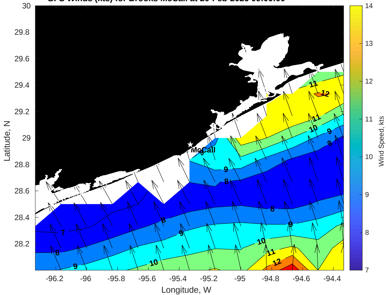
GFS Winds (kts) for Brooks McCall at 20-Feb-2026 09:00:00
