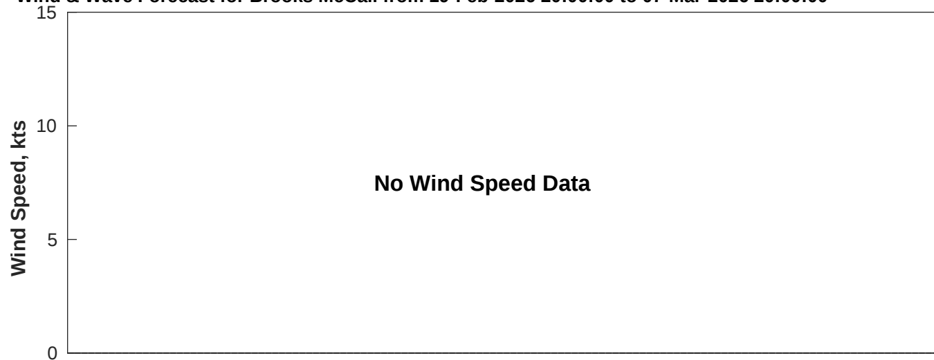
Wind & Wave Forecast for Brooks McCall from 19-Feb-2026 20:00:00 to 07-Mar-2026 20:00:00
