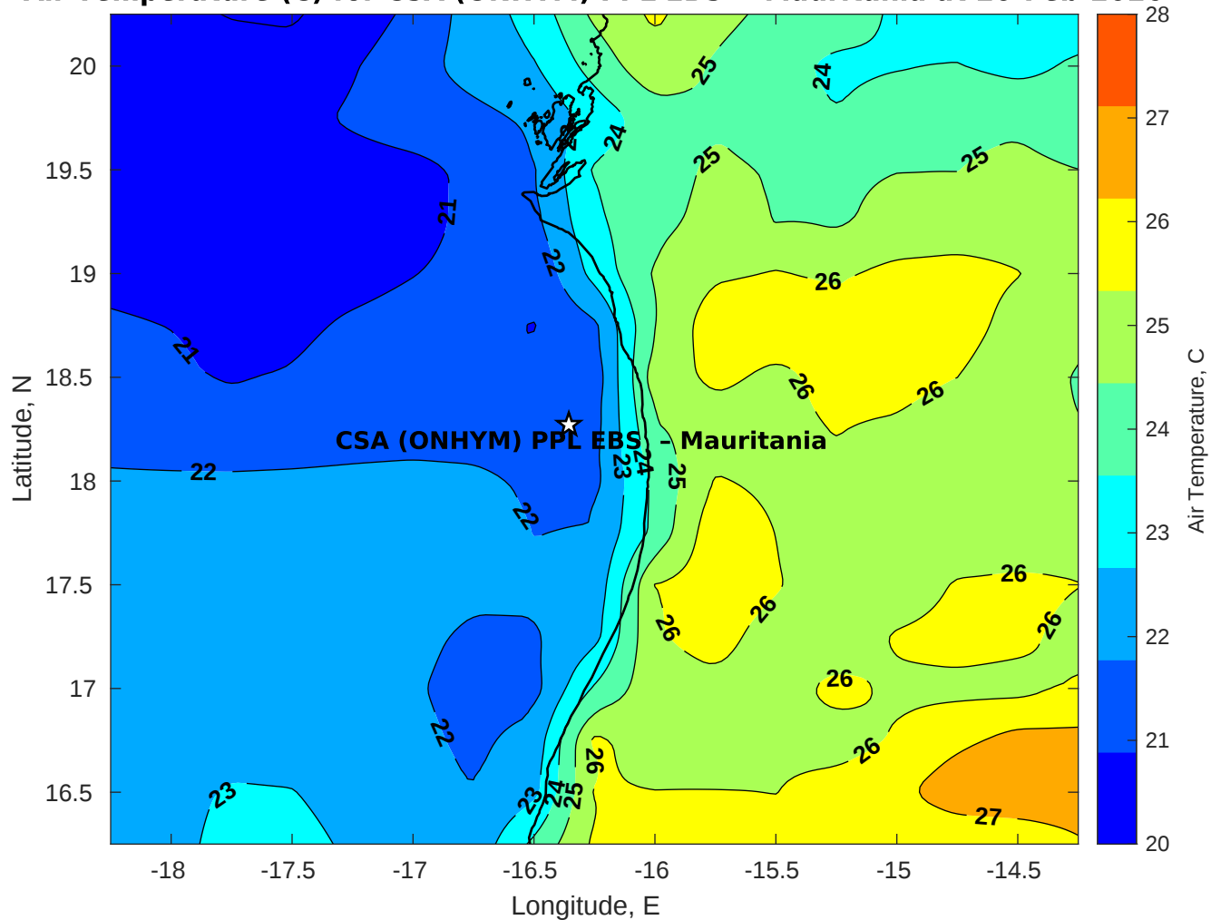
Air Temperature (C) for CSA (ONHYM) PPL EBS - Mauritania at 20-Feb-2026
