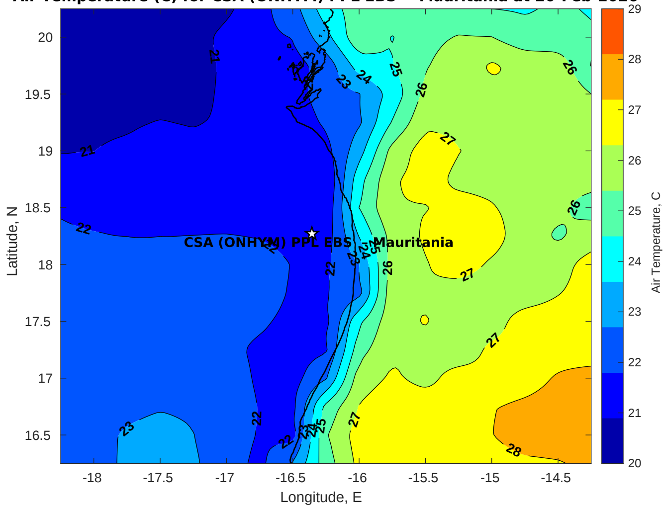
Air Temperature (C) for CSA (ONHYM) PPL EBS - Mauritania at 20-Feb-2026
