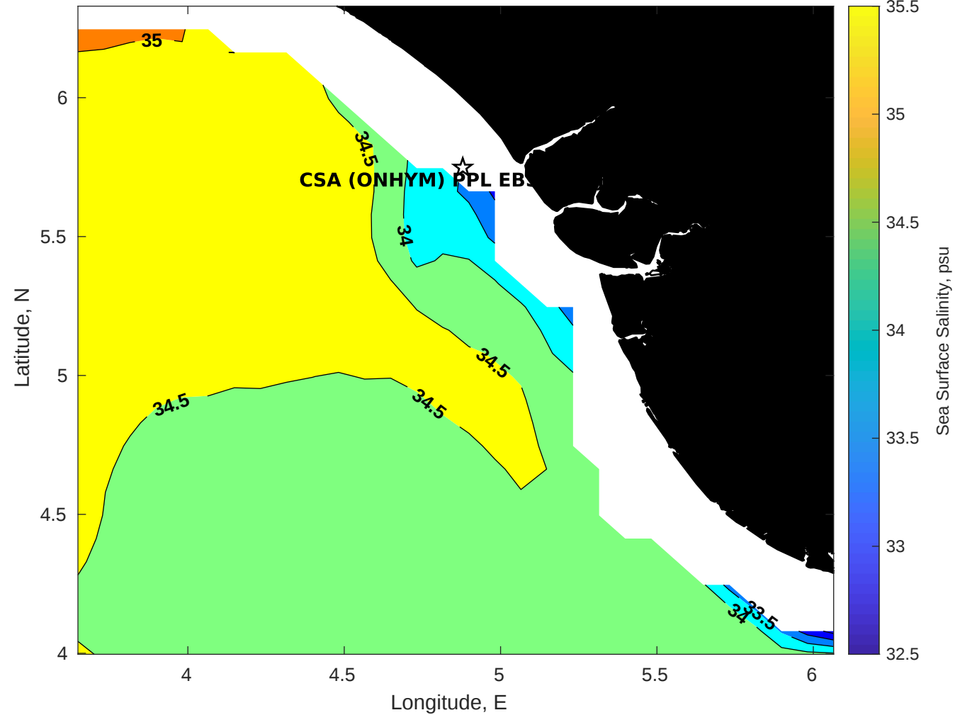
Surface Salinity for CSA (ONHYM) PPL EBS - Nigeria at 19-Feb-2026 00:00:00
