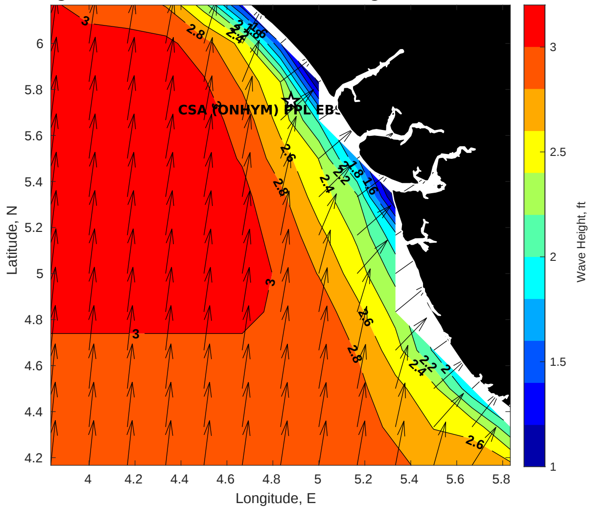
GFS Wave Height (ft) for CSA (ONHYM) PPL EBS - Nigeria at 20-Feb-2026 09:00:00
