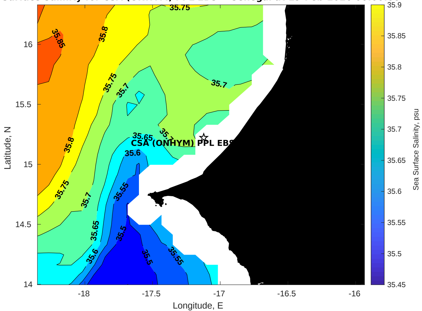
Surface Salinity for CSA (ONHYM) PPL EBS - Senegal at 19-Feb-2026 00:00:00
