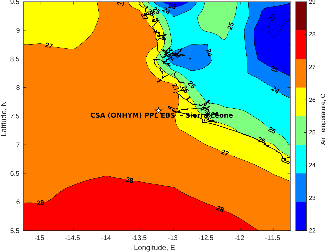
Air Temperature (C) for CSA (ONHYM) PPL EBS - Sierra Leone at 20-Feb-2026
