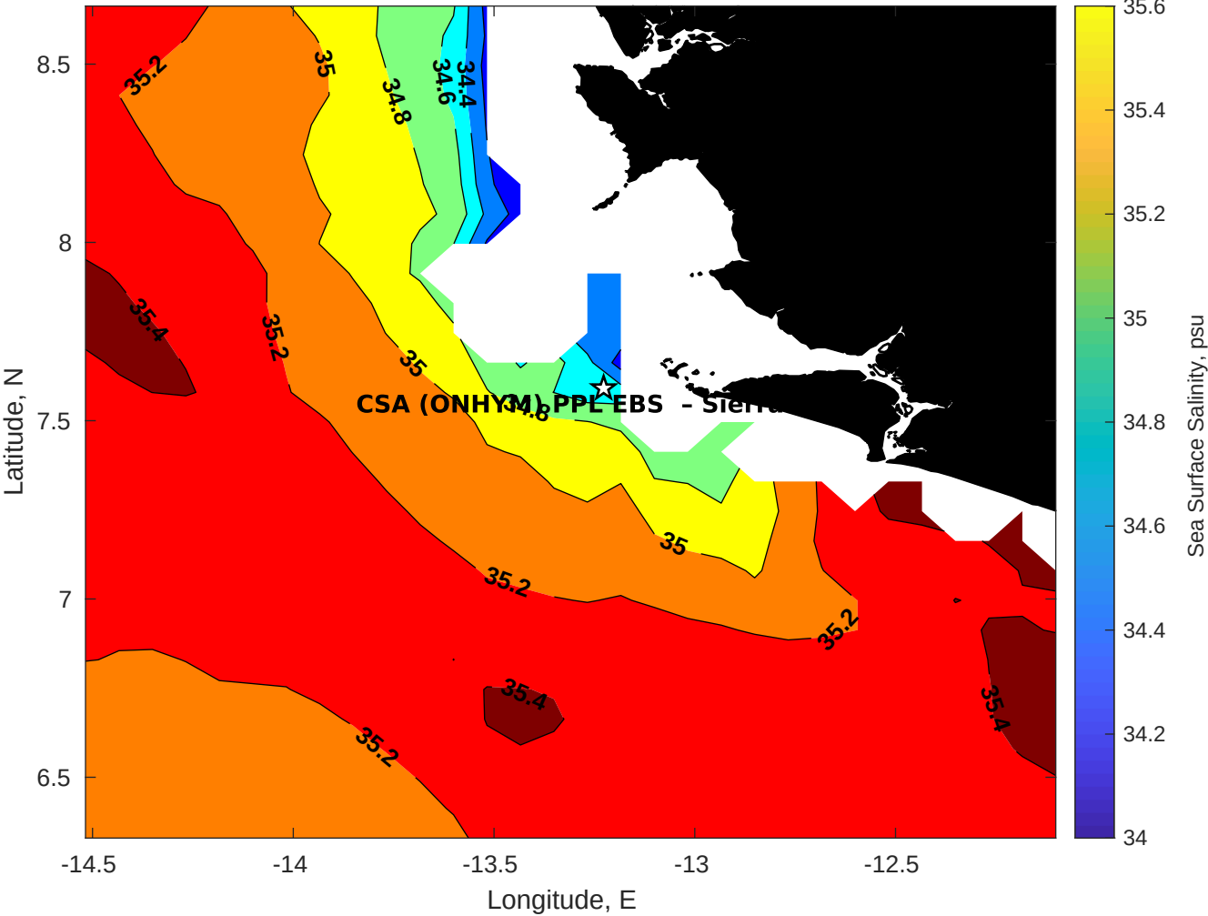
Surface Salinity for CSA (ONHYM) PPL EBS - Sierra Leone at 19-Feb-2026 00:00:00
