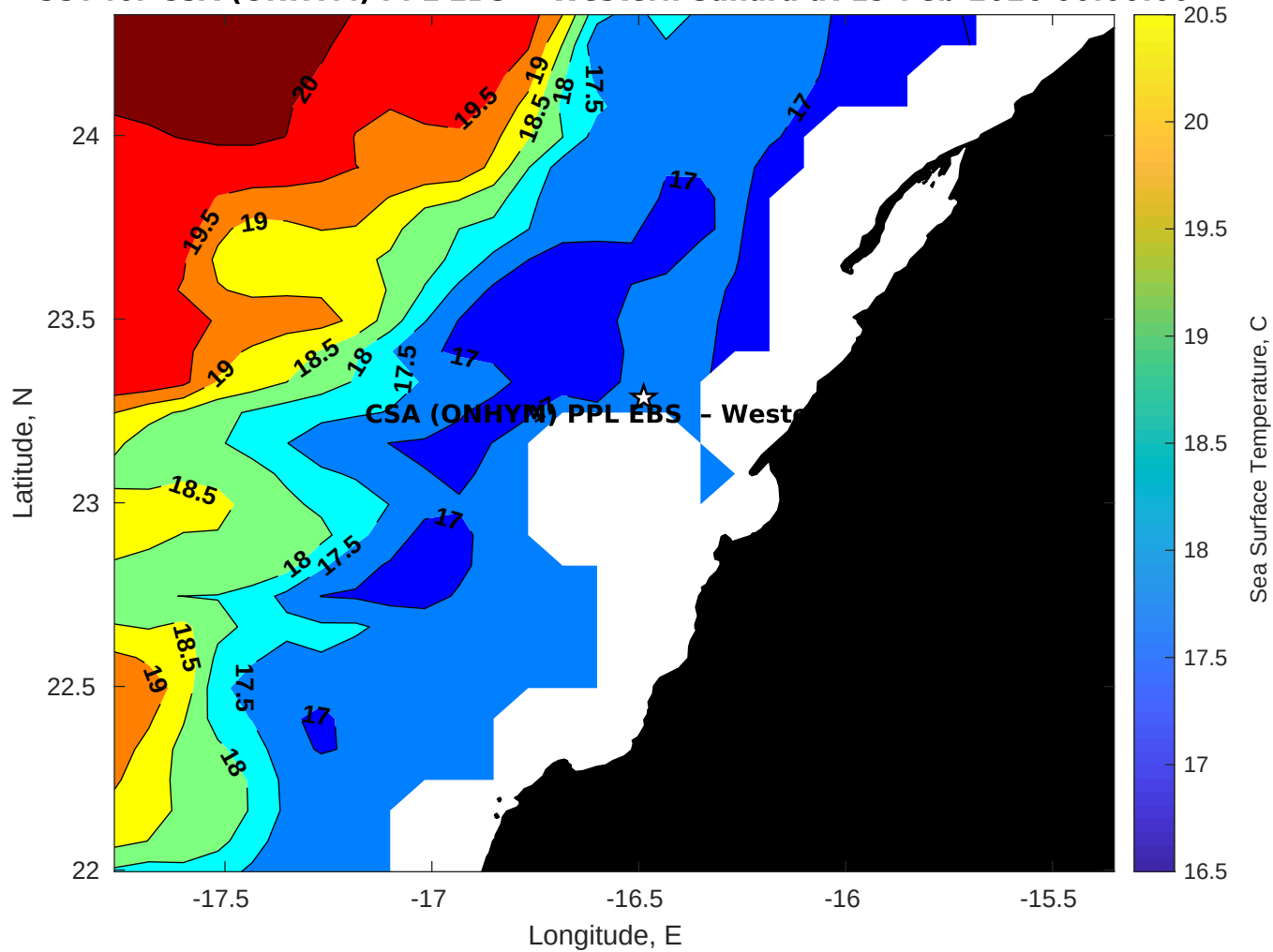
SST for CSA (ONHYM) PPL EBS - Western Sahara at 19-Feb-2026 00:00:00
