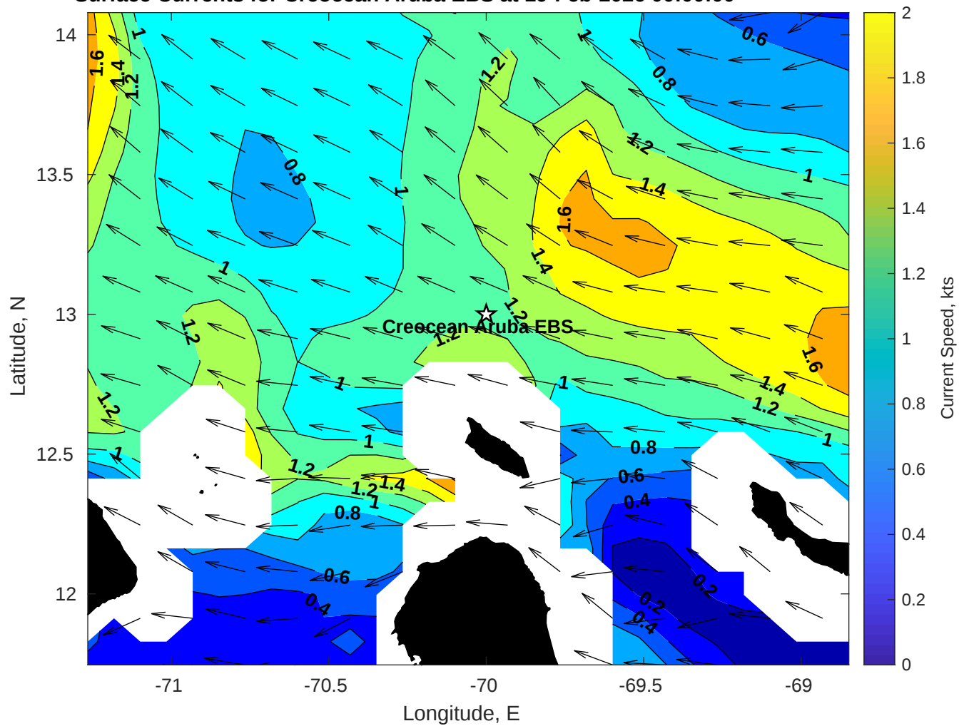
Surface Currents for Crecean Aruba EBS at 19-Feb-2026 00:00:00
