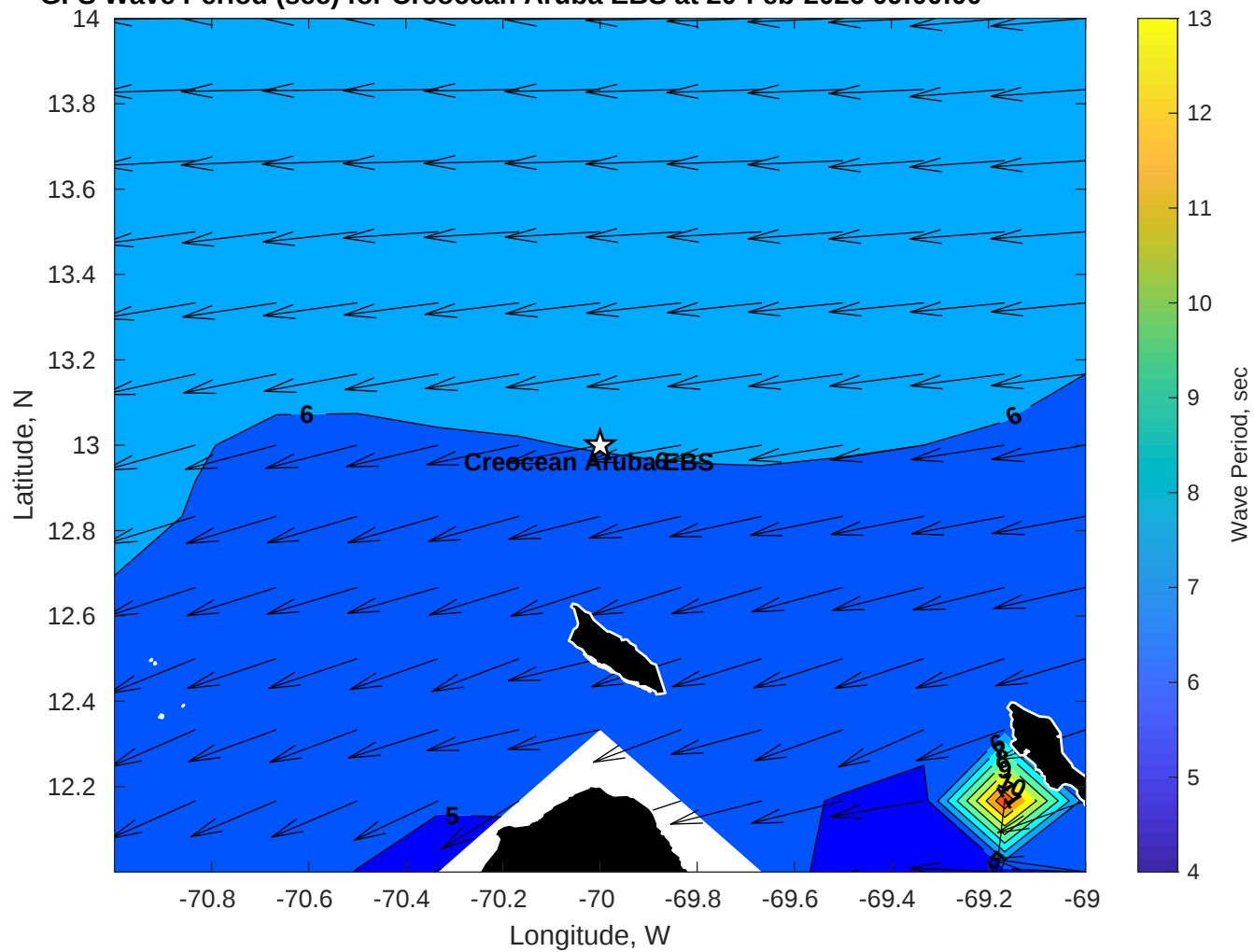
GFS Wave Period (sec) for Creoccean Aruba EBS at 20-Feb-2026 09:00:00
