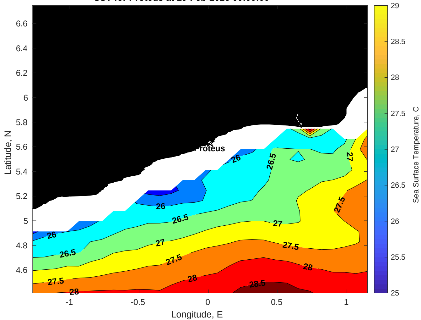
SST for Proteus at 19-Feb-2026 00:00:00
