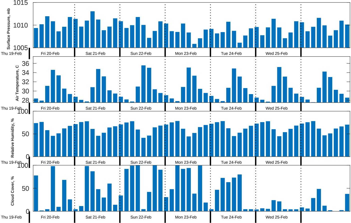
Met Forecast for Proteus from 20-Feb-2026 00:00:00 to 27-Feb-2026 00:00:00
