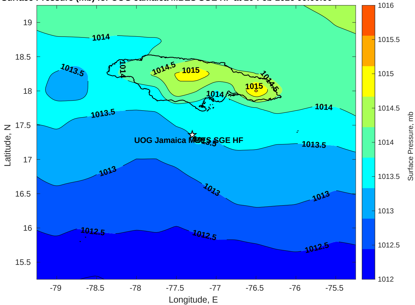
Surface Pressure (mb) for UOG Jamaica MBES SGE HF at 20-Feb-2026 00:00:00
