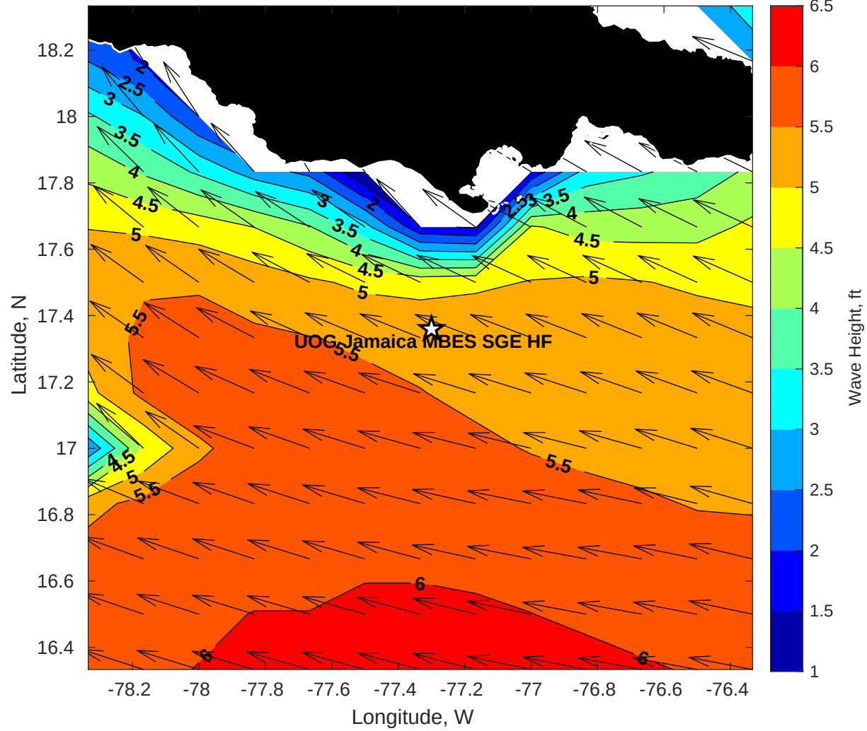
GFS Wave Height (ft) for UOG Jamaica MBES SGE HF at 20-Feb-2026 09:00:00
