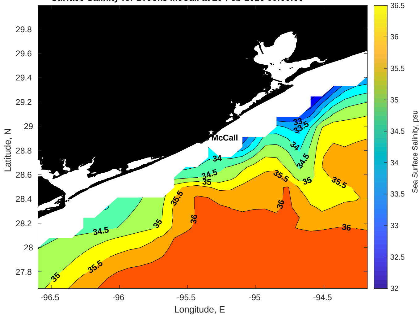
Surface Salinity for Brooks McCall at 20-Feb-2026 00:00:00
