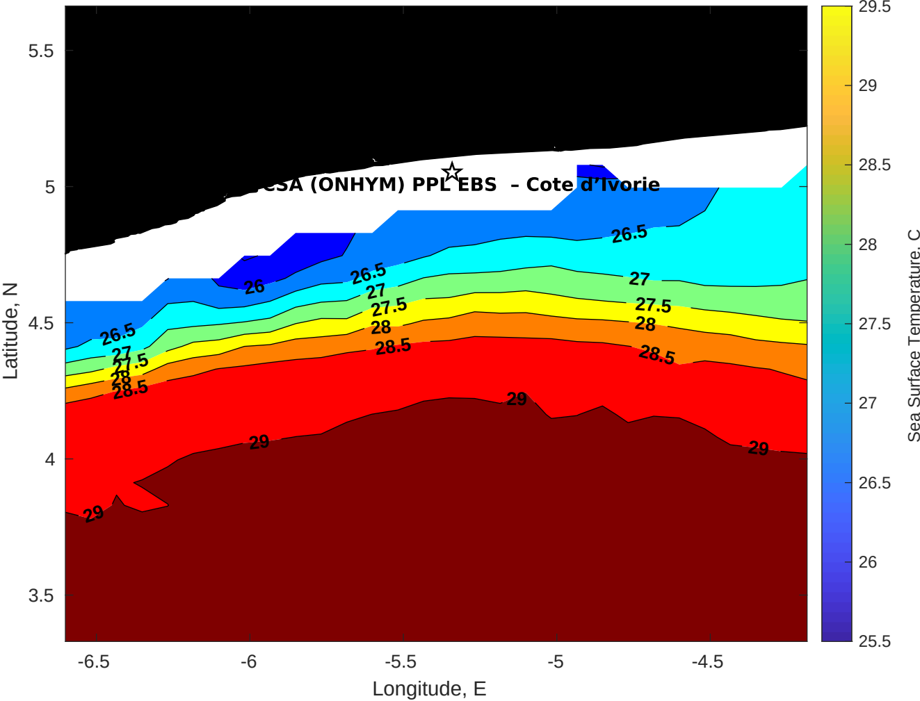
SST for CSA (ONHYM) PPL EBS - Cote d'Ivoire at 20-Feb-2026 00:00:00
