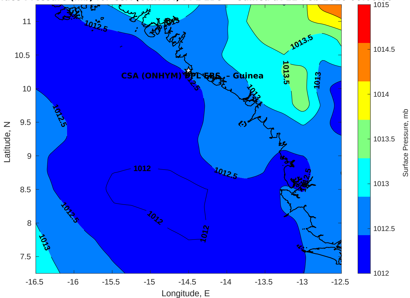
Surface Pressure (mb) for CSA (ONHYM) PPL EBS - Guinea at 22-Feb-2026 00:00:00
