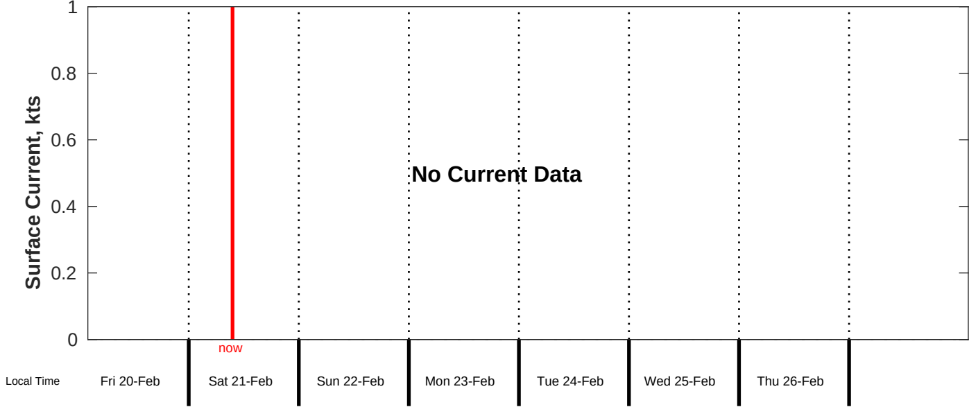
Surface Current Forecast for CSA (ONHYM) PPL EBS - Guinea from 20-Feb-2026 00:00:00 to 28-Feb-2026 00:00:00
