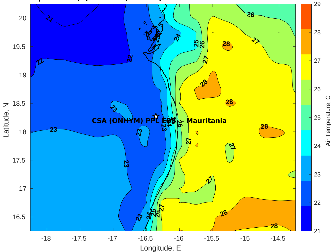
Air Temperature (C) for CSA (ONHYM) PPL EBS - Mauritania at 21-Feb-2026
