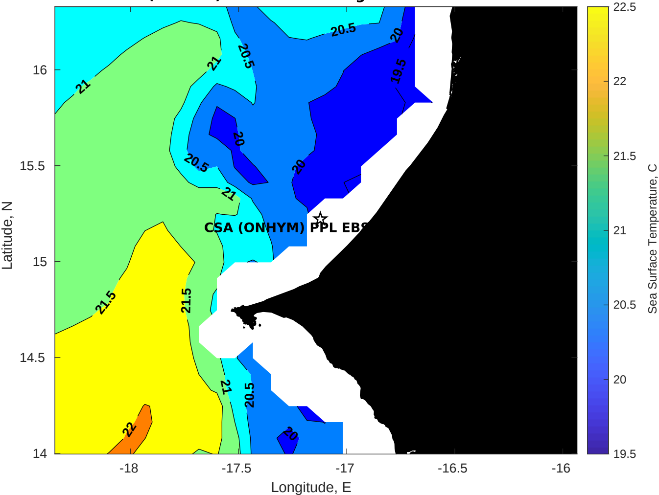
SST for CSA (ONHYM) PPL EBS - Senegal at 20-Feb-2026 00:00:00
