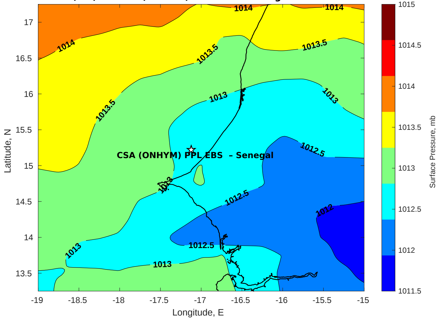
Surface Pressure (mb) for CSA (ONHYM) PPL EBS - Senegal at 22-Feb-2026 00:00:00
