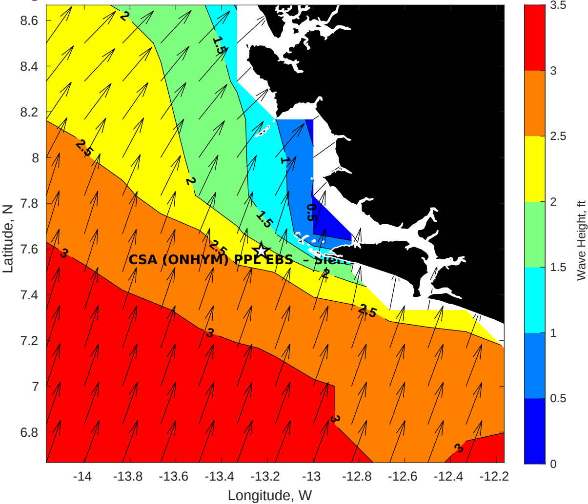
GFS Wave Height (ft) for CSA (ONHYM) PPL EBS - Sierra Leone at 21-Feb-2026 09:00:00
