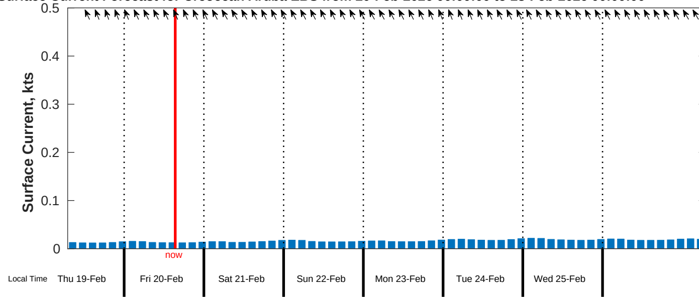
Surface Current Forecast for Creocean Aruba EBS from 20-Feb-2026 00:00:00 to 28-Feb-2026 00:00:00
