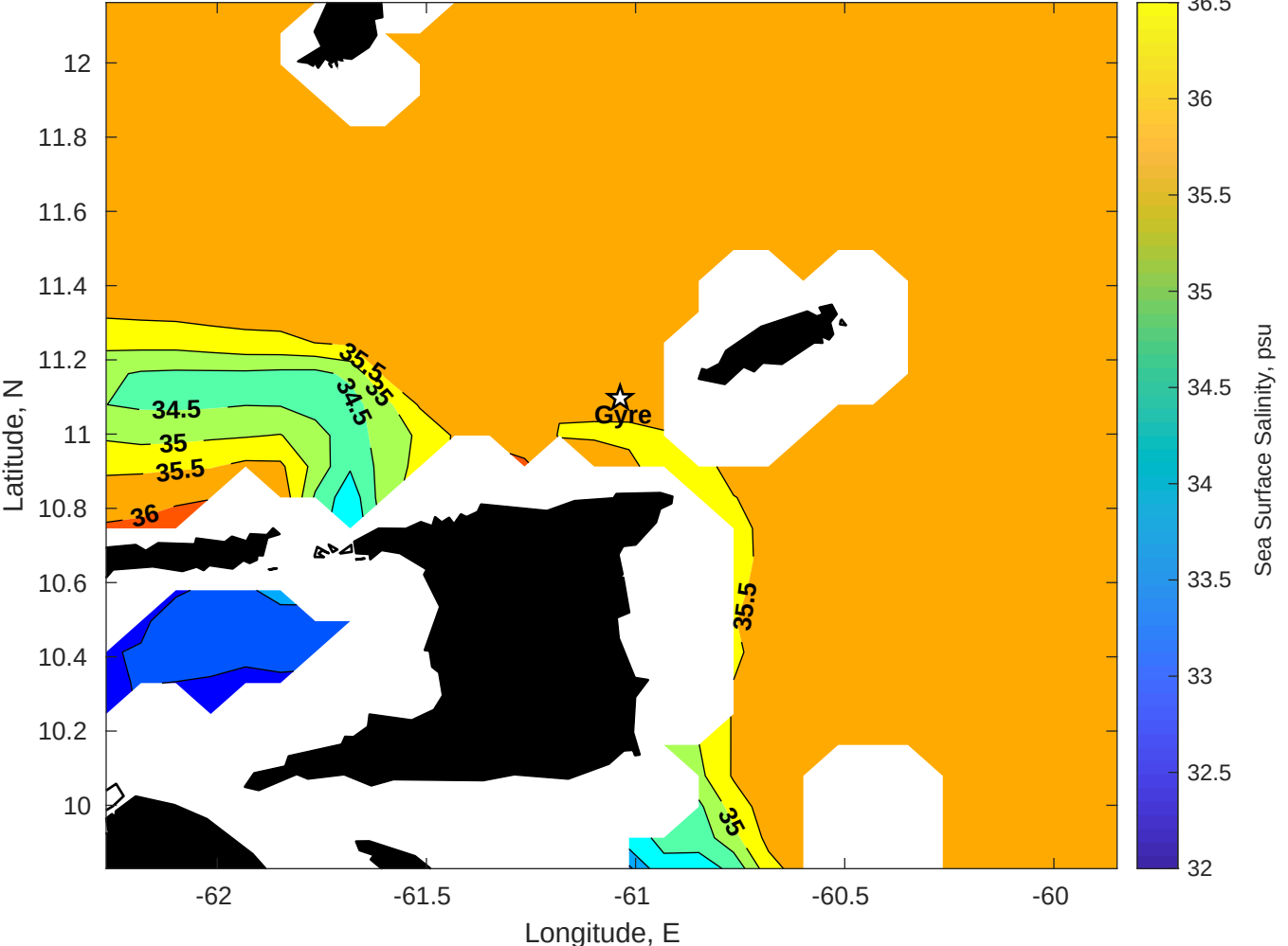
Surface Salinity for Gyre at 20-Feb-2026 00:00:00
