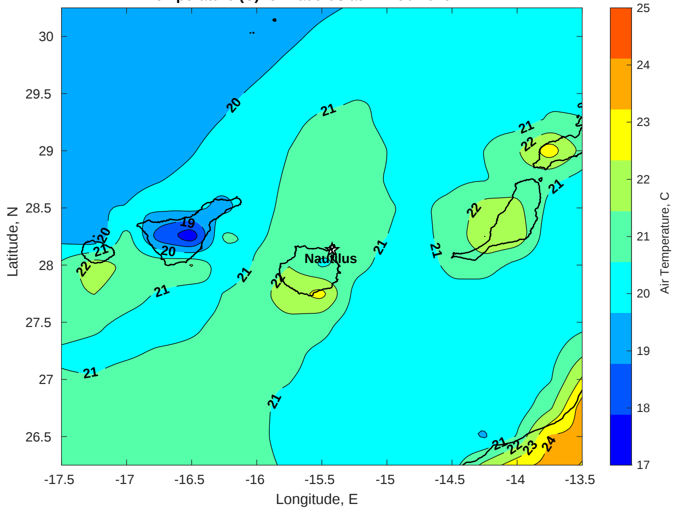
Air Temperature (C) for Nautilus at 21-Feb-2026
