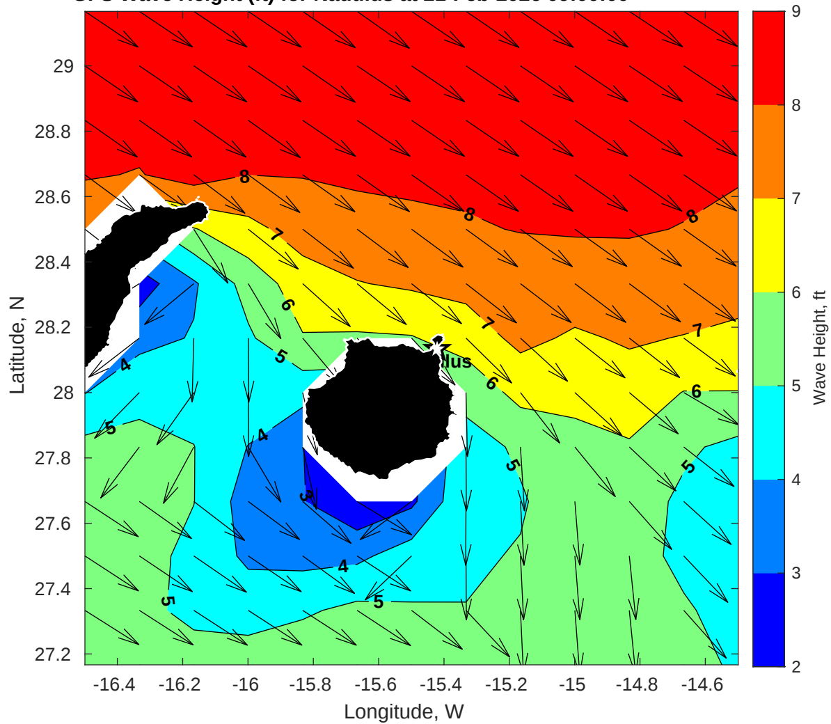
GFS Wave Height (ft) for Nautilus at 21-Feb-2026 09:00:00
