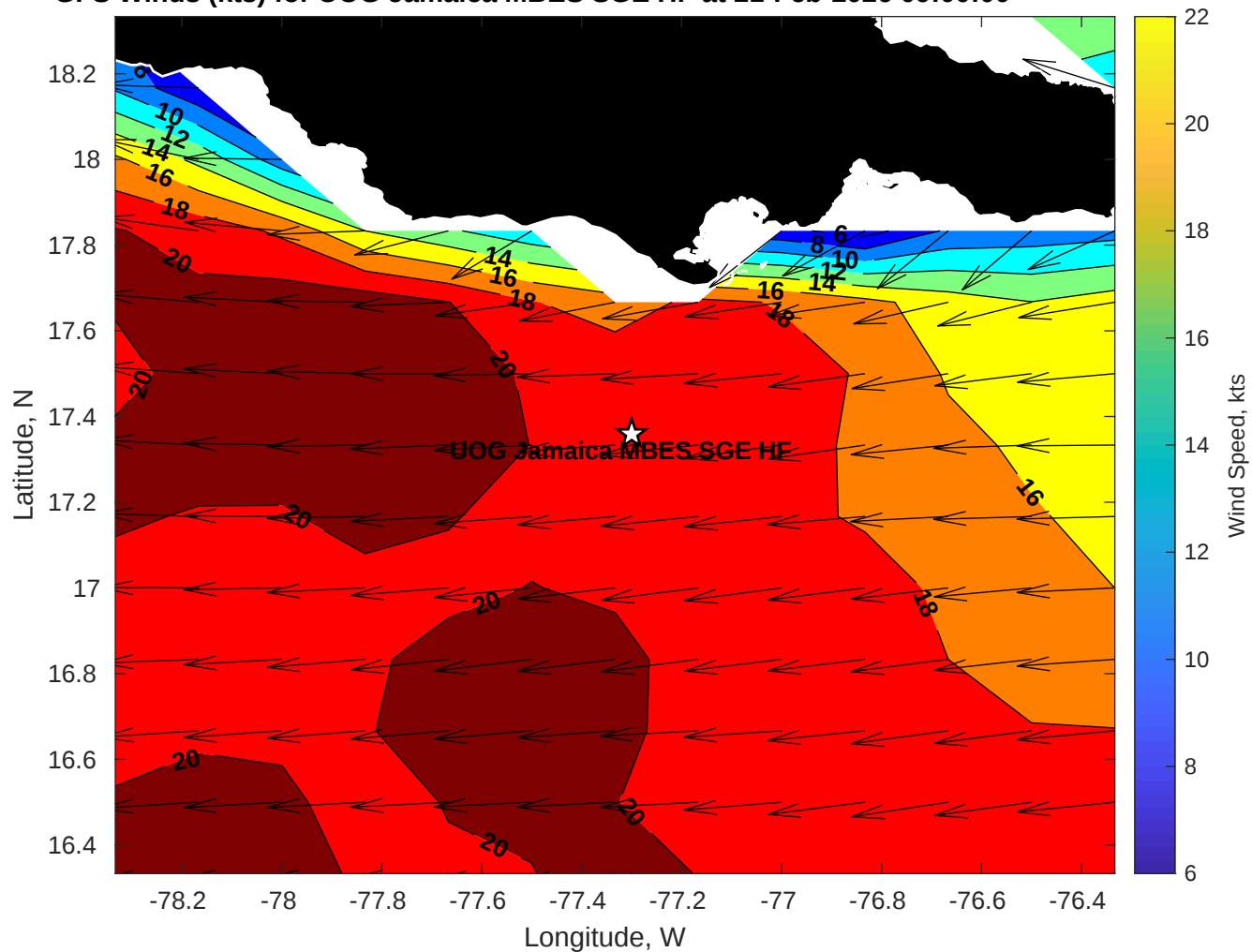
GFS Winds (kts) for UOG Jamaica MBES SGE HF at 21-Feb-2026 09:00:00
