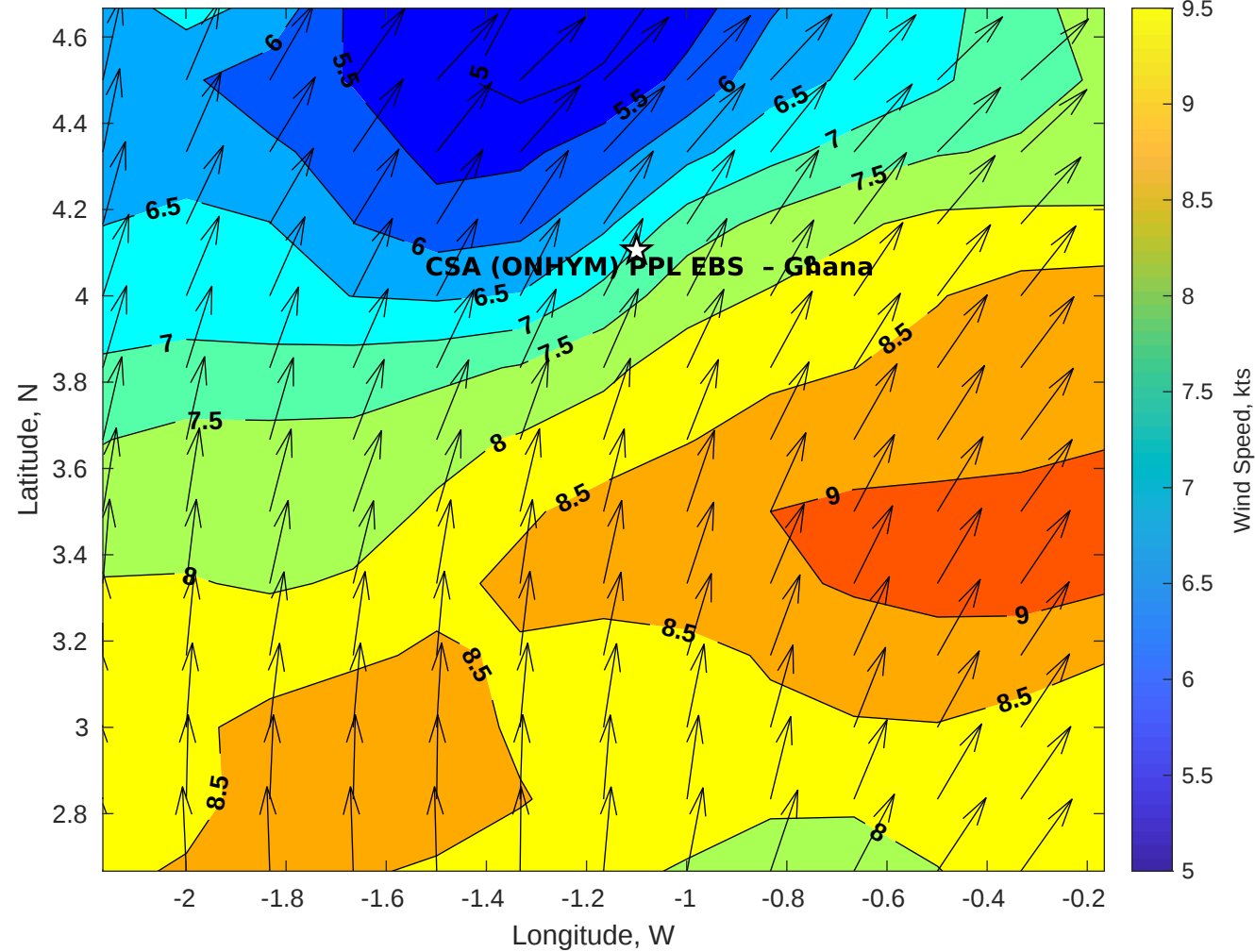
GFS Winds (kts) for CSA (ONHYM) PPL EBS - Ghana at 22-Feb-2026 09:00:00
