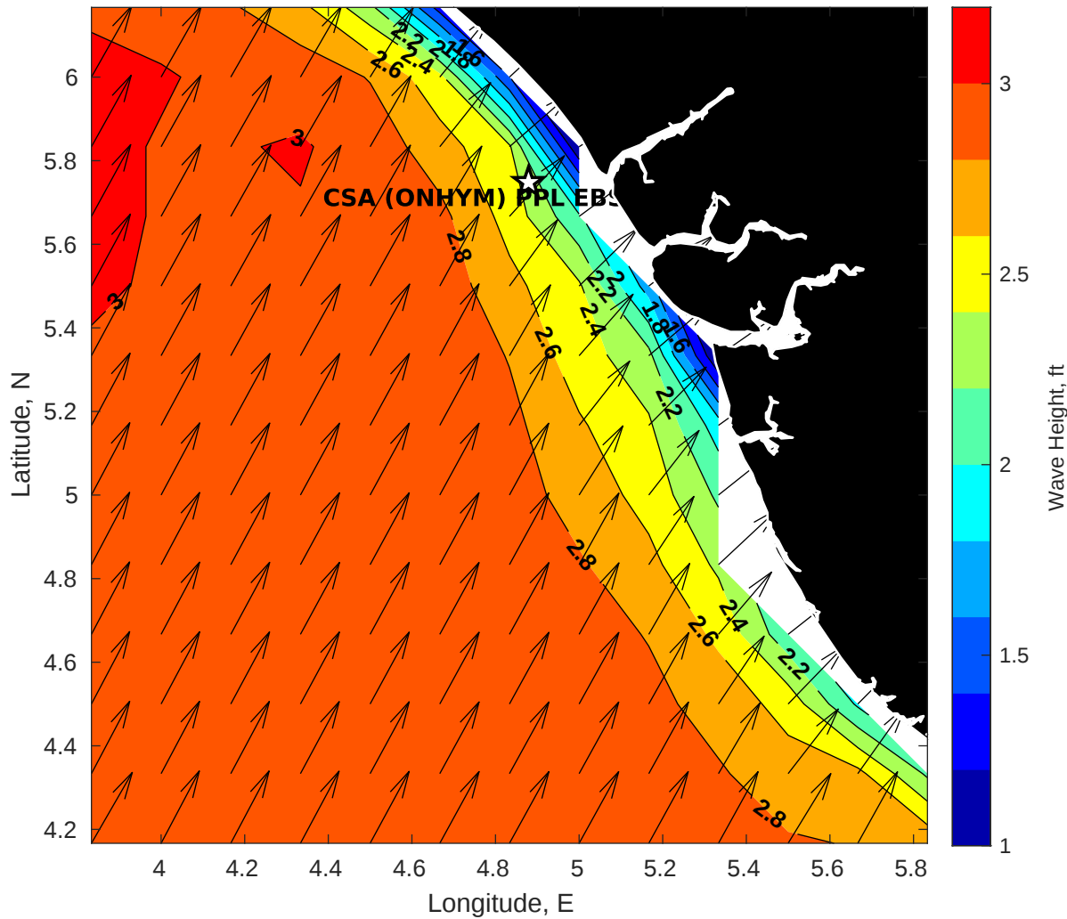
GFS Wave Height (ft) for CSA (ONHYM) PPL EBS - Nigeria at 22-Feb-2026 09:00:00
