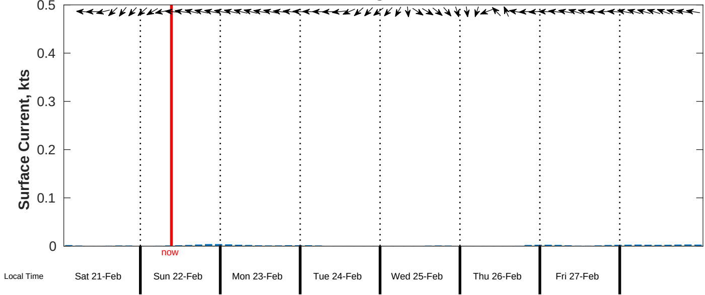
Surface Current Forecast for CSA (ONHYM) PPL EBS - Nigeria from 21-Feb-2026 00:00:00 to 01-Mar-2026 00:00:00
